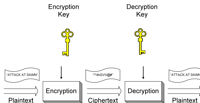
Figure 2: An Asymmetric Cryptosystem
